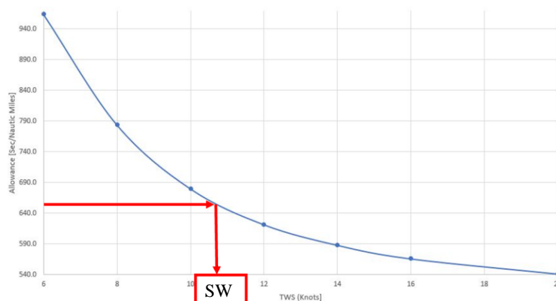
Figure 2: Performance Curve
